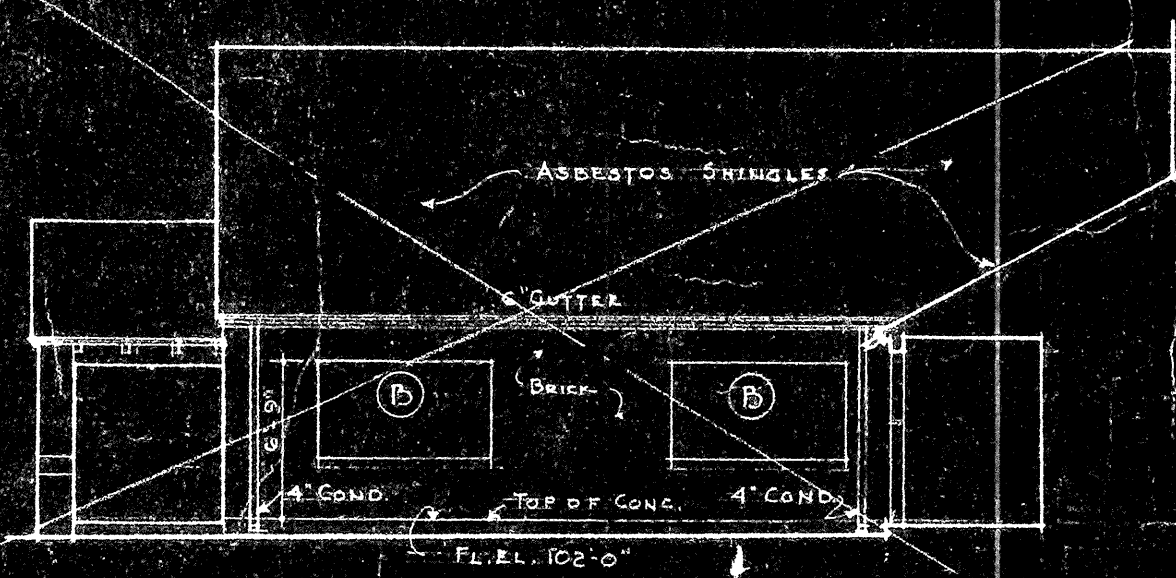
• NORTH ELEVATION OF PARISH HALL • SECTION 1/8"=1'-0"
