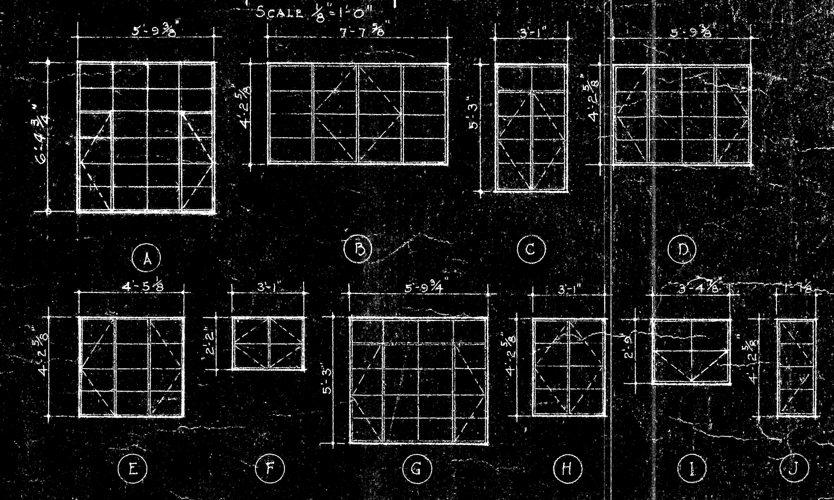
• WINDOW SCHEDULE • REVISOR: J. VAN DER BEEK
