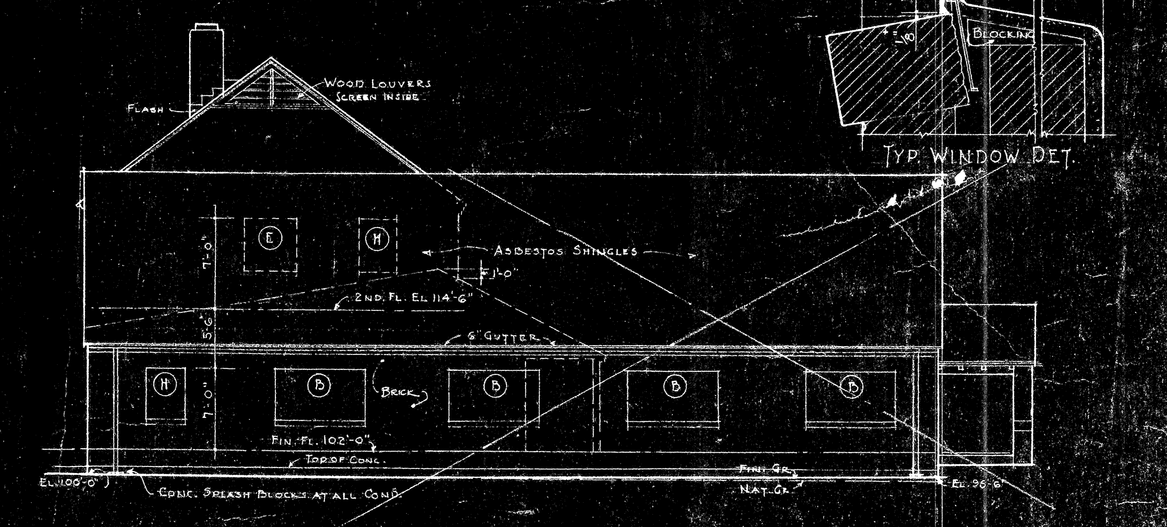
• SOUTH ELEVATION • SCALE 1/8"=1'-0"
